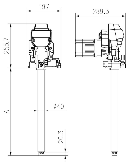
标准泵尺寸 Standalone pump, without oil tank (mm)
