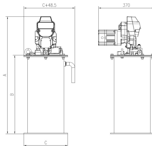
带桶尺寸 With tank dimensions(mm)
