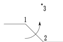
SPST Normally closed type
